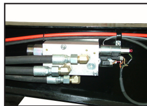
Trailer Mounted Electric Over Hydraulic Control Valve
