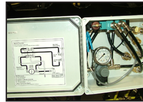
Lift Axle Control Box
