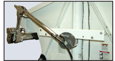
Roll Rite (shown) and Aero (not shown) Tarps with Lock out Sensor
