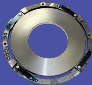
Ductile Iron Adapter Ring vs. Aluminum Strapped Center Plate
